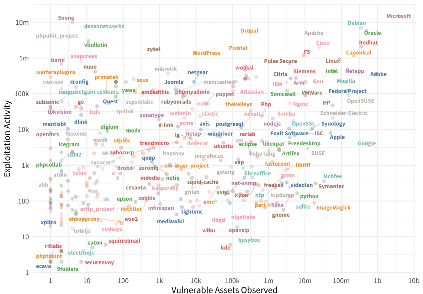
Figure 12: Major software vendors plotted according to the total number of vulnerabilities and exploitations observed
