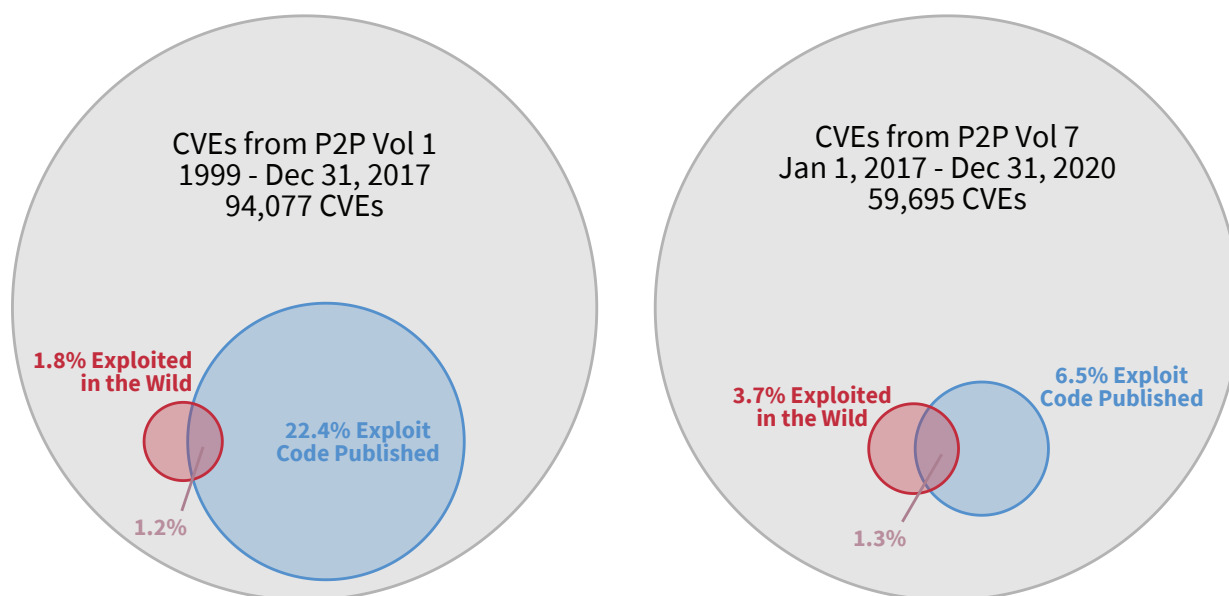
Figure 2: Proportion of published CVEs with exploit code and/or observed exploits in the wild
