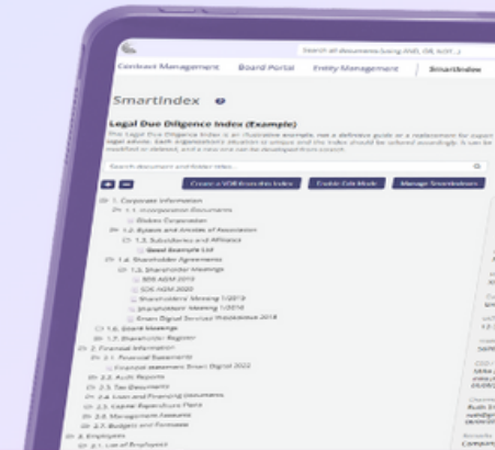
SmartIndex
